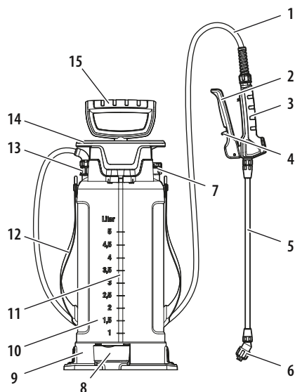
Parts of the pressure sprayer
